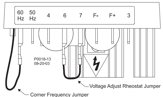
Figure 3 - Jumper Locations
